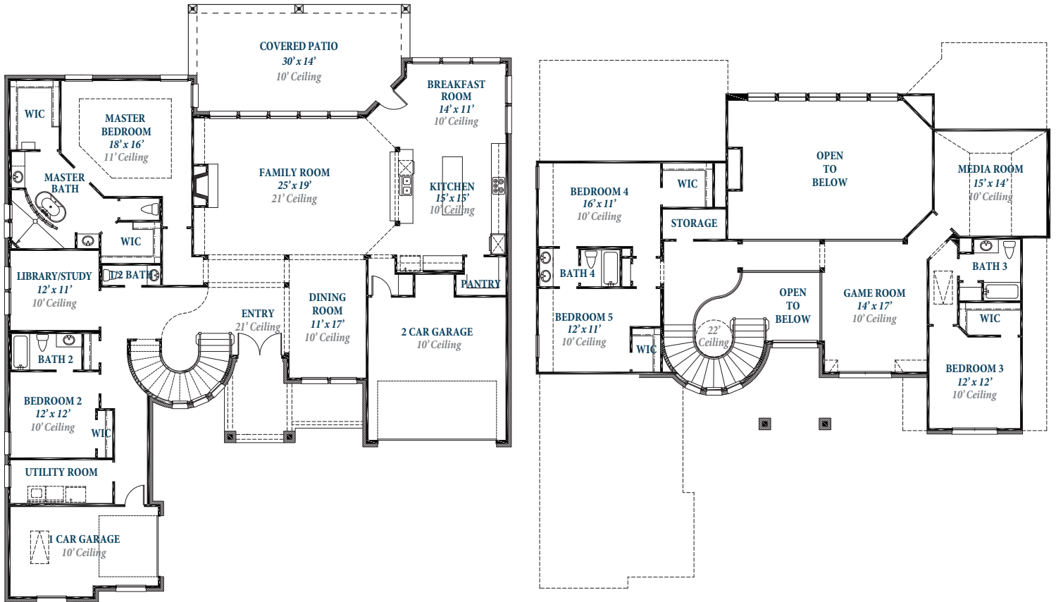
• FIRST FLOOR •
