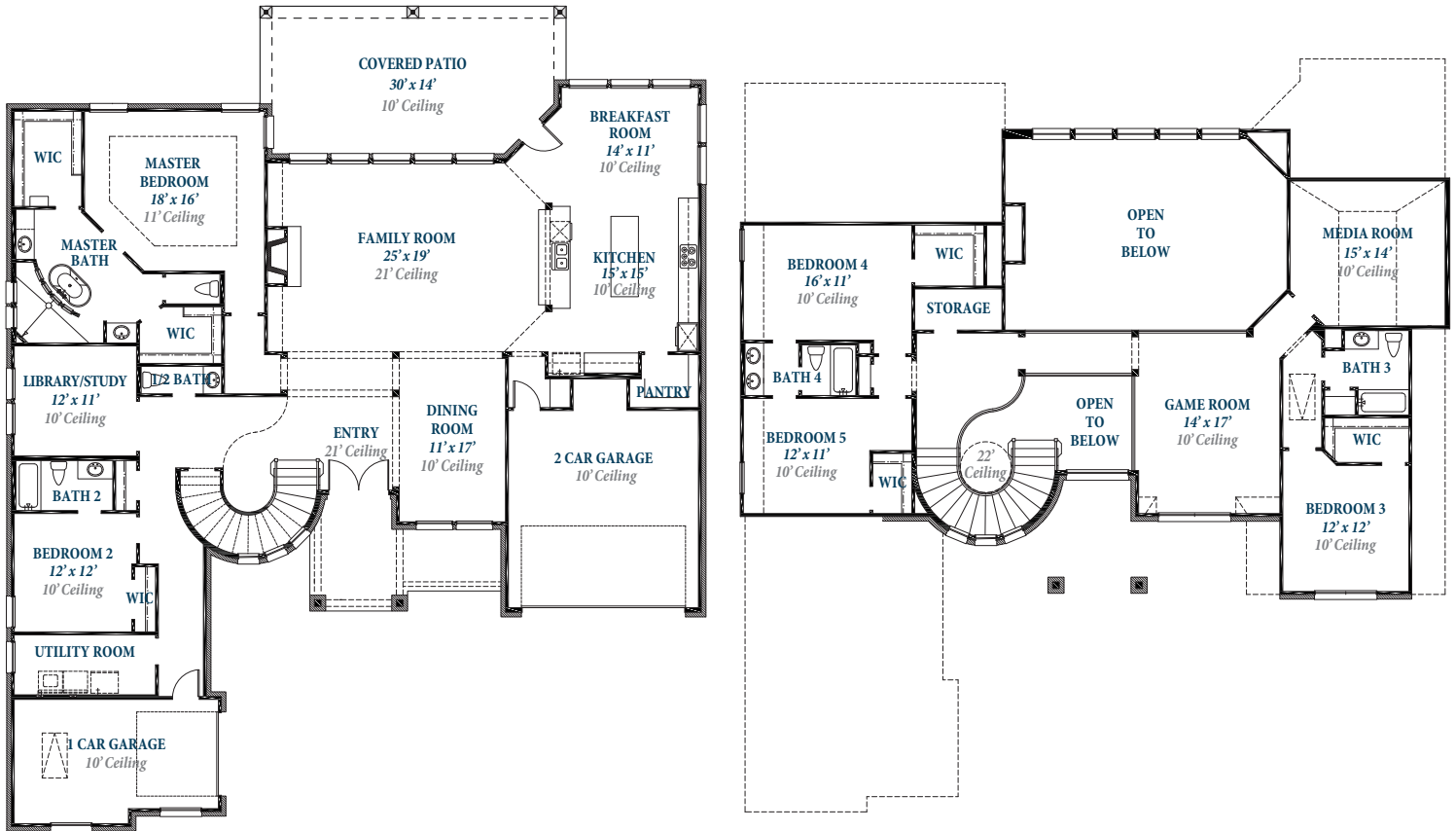
• FIRST FLOOR •
