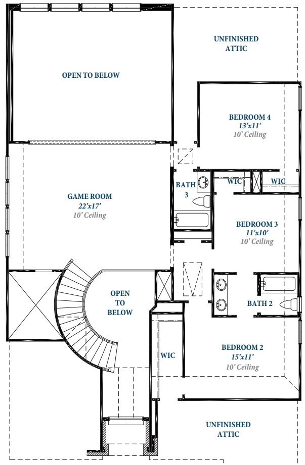
• SECOND FLOOR •
