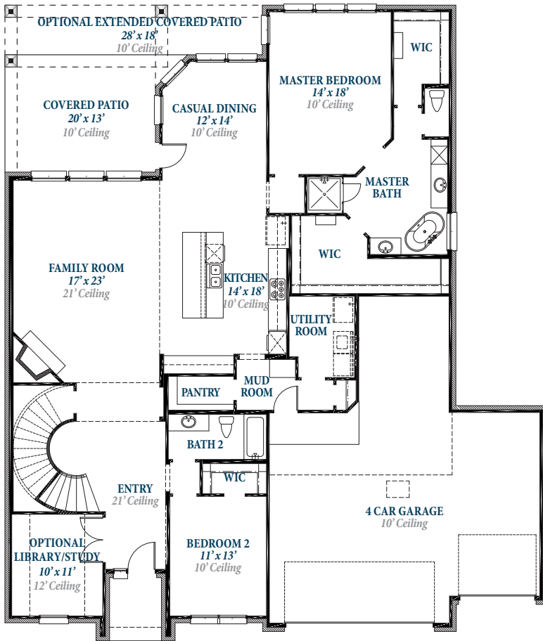
• FIRST FLOOR •
