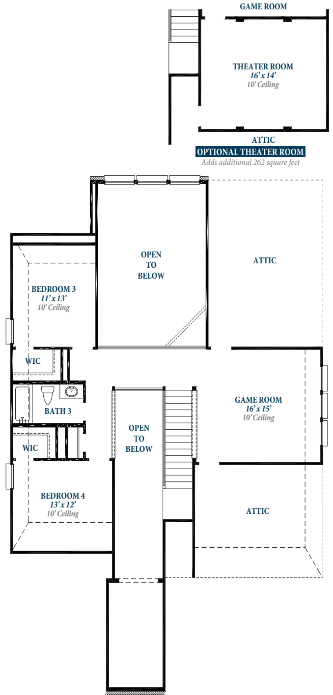
• SECOND FLOOR •
