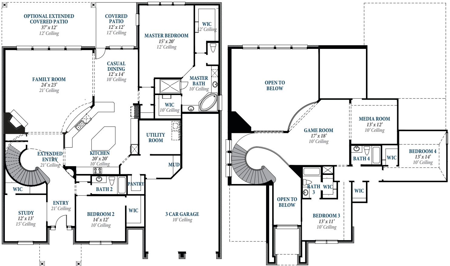
• FIRST FLOOR •
